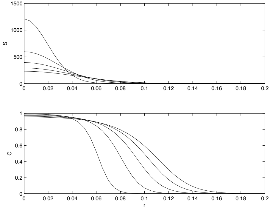
Figure 2: The distributions of the free-substrate S and enzyme-substrate complex C obtained by numerically integrating the full system given in equation (2.3) with initial data (2.4) (with the delta function being approximated by a tent function) are shown at times t = 2, 4, 6, 8, 10 . Other parameters are D = 10^{-4} , K_M = 11 , (k_1 = 1, k_2 = 1, k_{-1} = 10) , E_0 = 1 , S_0 = 3 , I \equiv 0 . Numerically obtained solutions of the reduced system (2.5) are graphically indistinguishable from those obtained by solving the full system (2.3).
