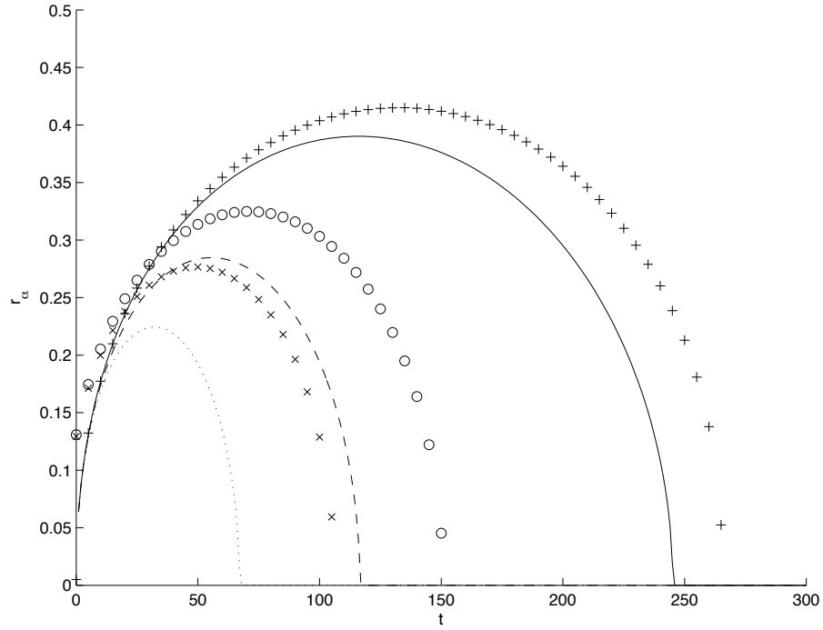
Figure 3: The value r_\alpha such that \alpha = S_q(r_\alpha, t) is determined by solving equations (2.5) with initial data (2.4) with \alpha = 1/4\pi for differing values of K_M and compared to analytical approximations obtained from (3.16) with k = k_2 E_0 / K_M , representing a lower bound on the position of the substrate edge. The data points \times , \circ and + denote the position of the leading substrate edge determined by numerically solving the full system of equations with K_M taking values 11, 21 and 51 respectively. The corresponding analytical approximations (dotted, dashed and solid lines) obtained from equation (3.16) are shown. The remaining parameter values are k_2 = 1 , S_0 = 3 , E_0 = 1 , D = 10^{-4} .
