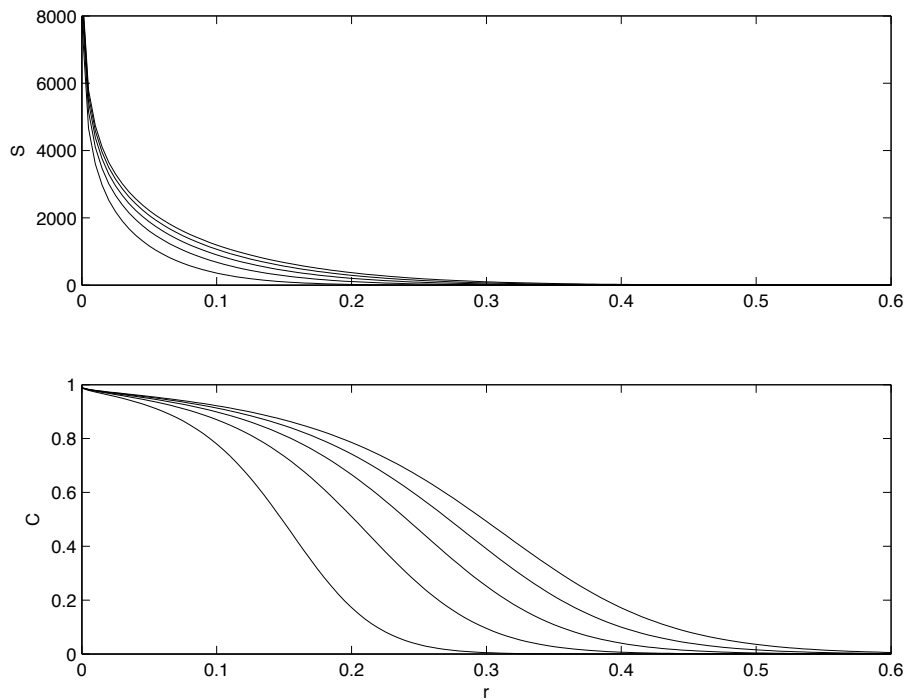
Figure 5: The distributions of the free-substrate S and enzyme-substrate complex C obtained by numerically integrating the full system given in equation (2.3) with initial data (2.4) (with the delta function being approximated by a tent function) are shown at times t = 40, 80, 120, 160, 200 . Other parameters are D = 10^{-4}, k_1 = 1, k_2 = 1, k_{-1} = 100, (K_M = 101), E_0 = 1, S_0 = 3, I_0 = 1
