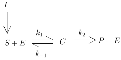
Figure 1: The enzyme-substrate reaction with substrate input
