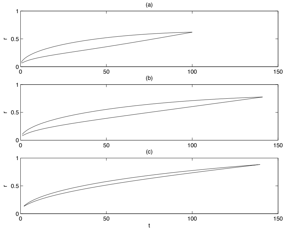
Figure 4: The region in r - t -space inside which the error E_M := 2(S_q - S)/(S_q + S) > 0.2 and the substrate concentration S > 10^{-6} . The inner and outer bounds of this region, corresponding to the position where E_M = 0.2 and S = 10^{-6} respectively, are plotted over time for parameter values k_1 = 1, k_2 = 1, S_0 = 3, E_0 = 1, D = 10^{-4} with (a) K_M = 11(k_1 = 10) , (b) K_M = 21(k_1 = 20) , and (c) K_M = 51(k_1 = 50)
