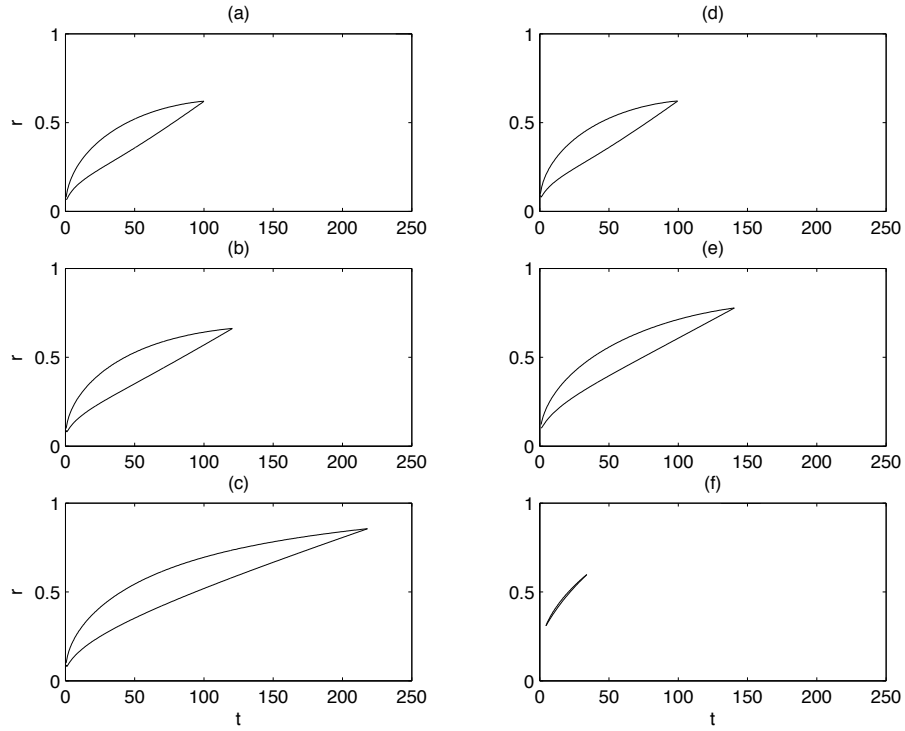
Figure 7: Equations (2.3) and (2.5) are solved numerically giving rise to an annular region expanding from the origin inside which the error E_M = 2(S_q - S)/(S_q + S) > 0.2 and the substrate concentration S > 10^{-6} . The inner and outer boundaries, corresponding to the position where E_M = 0.2 and S = 10^{-6} respectively, are plotted over time for parameter values k_1 = 1, k_2 = 1, S_0 = 3, E_0 = 1, D = 10^{-4} with (a) I_0 = 0, K_M = 11 , (b) I_0 = 0.1, K_M = 11 , (c) I_0 = 1, K_M = 11 , (d) I_0 = 10^{-3}, K_M = 11 , (e) I_0 = 10^{-3}, K_M = 21 , and (f) I_0 = 10^{-3}, K_M = 101 .
