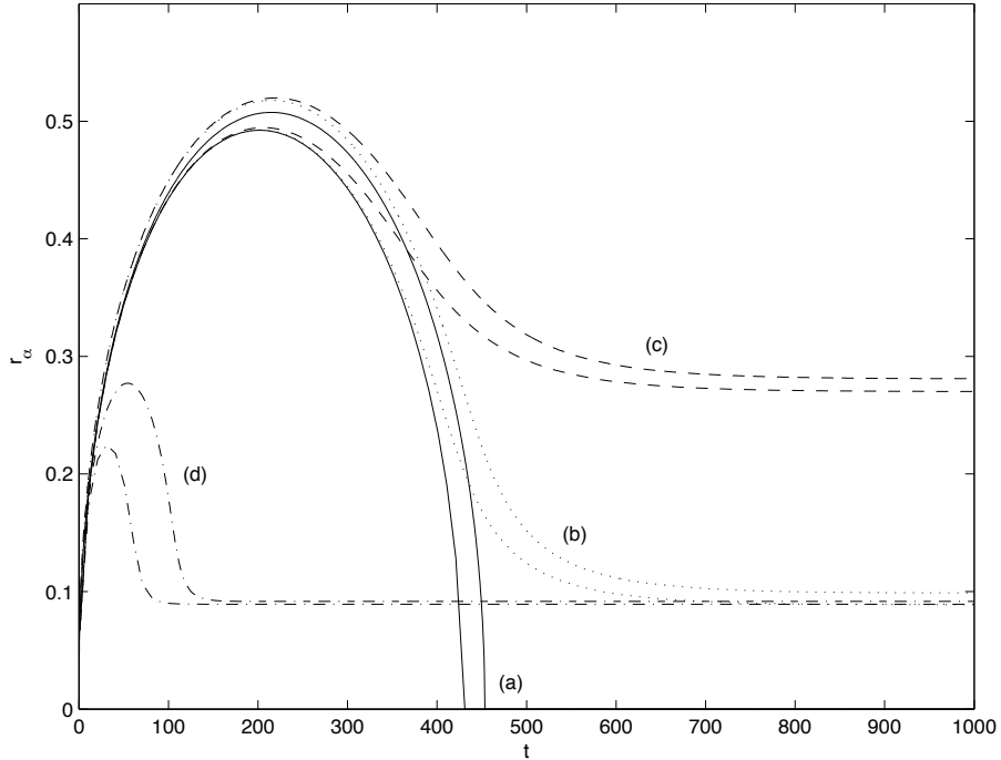
Figure 6: The value of r_\alpha for which \alpha = u_I(k_2 E_0 / K_M, r_\alpha, t) where u_I is defined in equation (4.18) is compared to that obtained by numerically solving the full system (2.3) for different input rates I_0 . The position of the leading edge obtained by solving the reduced system (2.5) is graphically indistinguishable from that obtained by solving the full system. The leading edge value \alpha is taken to be \frac{1}{4\pi} and the remaining parameter values are D = 10^{-4} , k_1 = 1 , k_2 = 1 , E_0 = 1 , S_0 = 3 with (a) I_0 = 0 , K_M = 101 , (b) I_0 = 10^{-4} , K_M = 101 , (c) I_0 = 10^{-3} , K_M = 101 and (d) I_0 = 10^{-3} , K_M = 11 . In each case, the higher curve denotes the position of the leading edge obtained through numerical integration of (2.3) and the lower curve denotes the lower bound obtained by solving equation (4.18).
