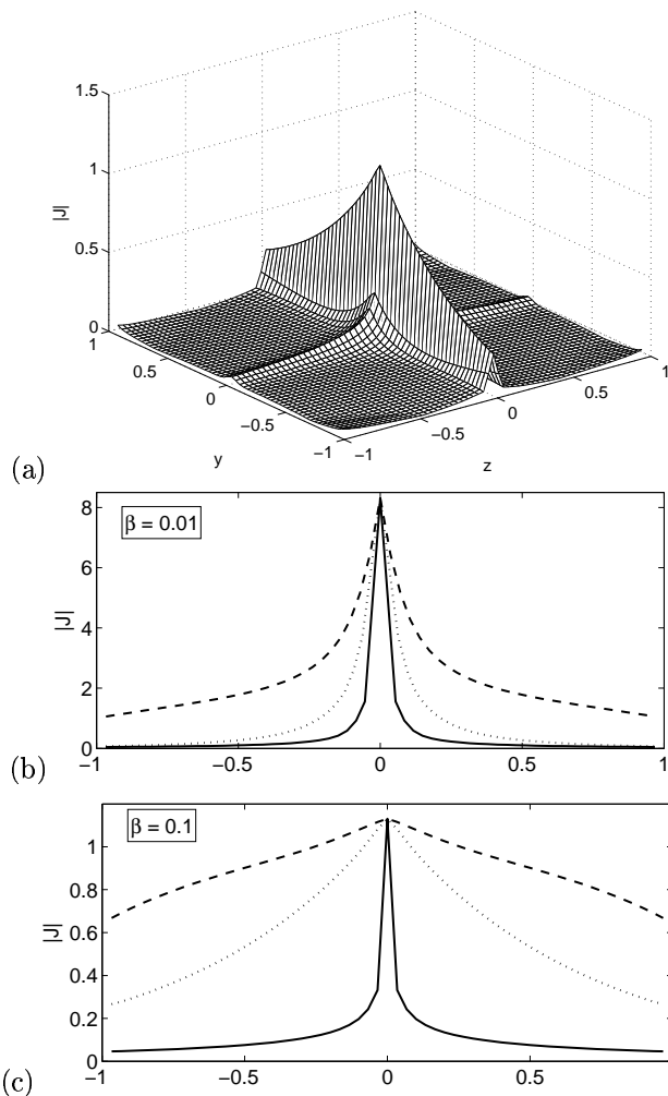
FIG. 6: (a) Modulus of the current plotted in the x = 0 plane demonstrating the spreading along the spine and fan, for N = 30 , \kappa = 1/2 and \beta = 0.1 . (b), (c) Current modulus along the spine (solid line) and along the x (dashed) and y (dotted) directions in the fan plane, showing the spreading of the current sheet, for (b) \beta = 0.01 and (c) \beta = 0.1 .
