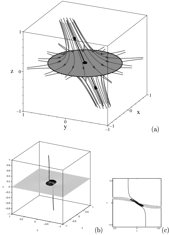
FIG. 1: (a) Schematic of the perturbed null point given by Eqs. (9,10); the black field line is the spine, and the grey disk represents the orientation of the fan plane. (b) Isosurface of the current magnitude at J_{max}/3 , for the 3D null point collapse, with \kappa = 1/2 , N = 30 , \beta = 0.01 . The black line is the spine, and the grey grid represents the fan plane, and (c) a close-up in the yz -plane.
