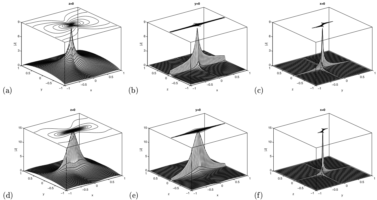
FIG. 3: Plots of |J| for the isotropic ( \kappa = 1/2 ) 3D null in the (a) xy -plane, (b) xz -plane and (c) yz -plane, for N = 30 and \beta = 0.01 . Overlaid on the top of the domain in each case is a contour plot of |J| , with the same contour levels plotted in each frame. (d-f) The same plots for an anisotropic null with \kappa = 1/4 .
