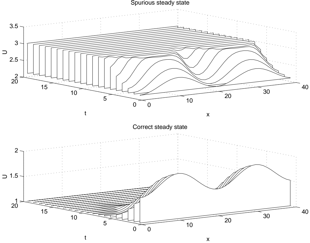
Figure 2: Spurious and correct steady states for the PIVP.
