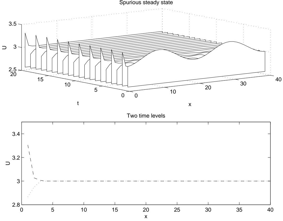
Figure 3: Spurious non-uniform steady state for the IBVP.
