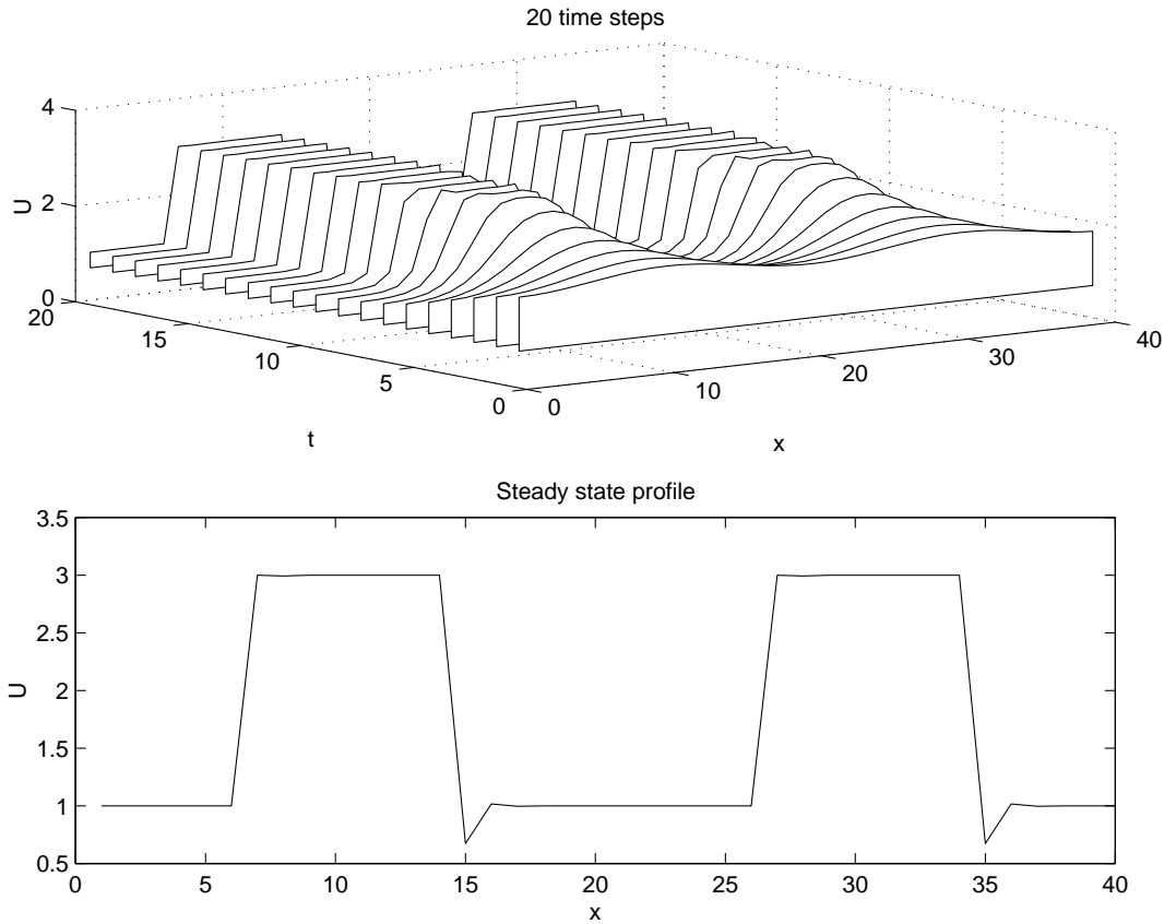
Figure 4: Stable steady state with jumps.
