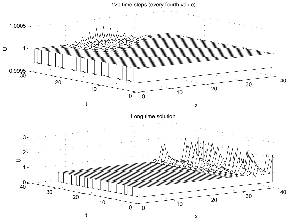
Figure 5: Spurious long term behaviour on the IBVP caused by nonnormality.
