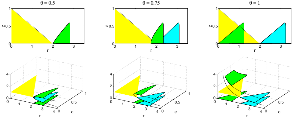
Figure 1: Stable parameter ranges in the (r, c) -plane for steady states of the \text{RK}(\theta) methods with \theta = 0.5, 0.75, 1.0 on the PIVP with (3). On the bottom row the vertical axis shows the magnitude of the steady state solution.
